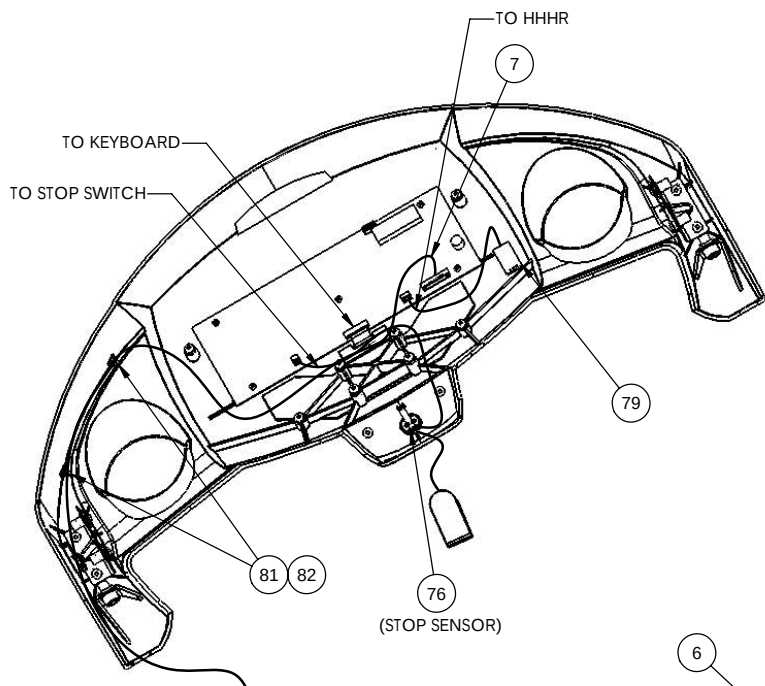
DISPLAY WIRING DETAIL
