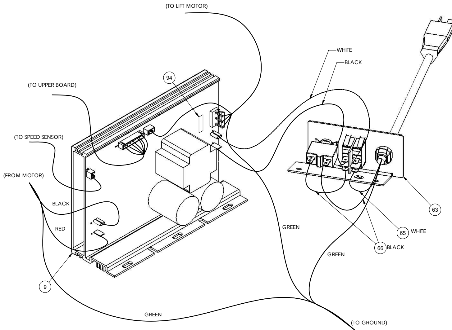
WIRING DETAIL
